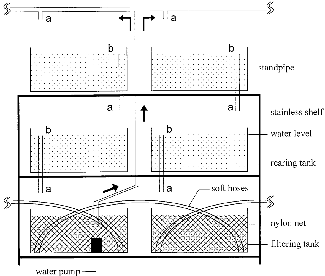
FIGURE 2.—Diagram of the recirculating-water systems (iterative aquaria excluded); arrows indicate the direction of flow, (a) indicates inflow locations, and (b) indicates outflow locations. In each of the four systems, the 14 rearing aquaria were situated at the upper and middle levels, and the 5 filtering aquaria were situated at the bottom level. Recirculated water was pumped from the bottom level to the top level and returned by gravity flow to the bottom level. The filtering aquaria were connected by soft hoses and were filled with nylon netting that served as the filters. All the aquaria were aerated.
